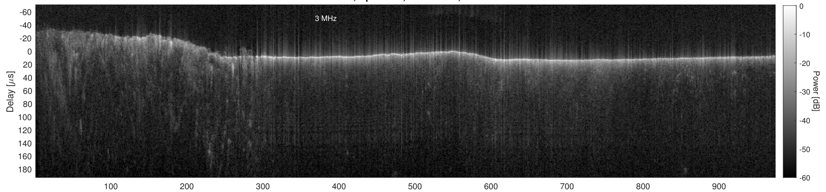
Orbit 16453, Cluttergram
