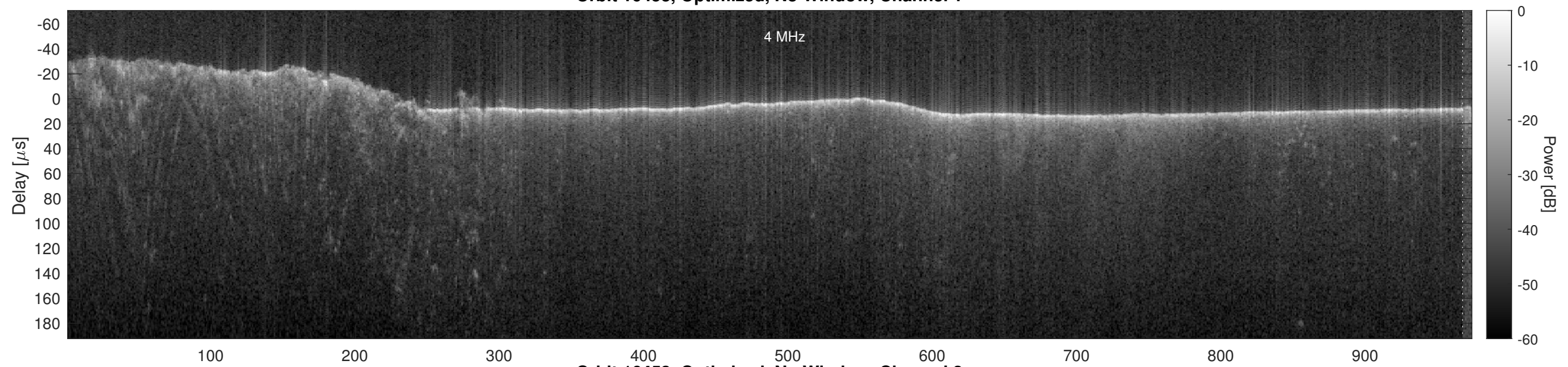
Orbit 16453, Optimized, No Window, Channel 2
