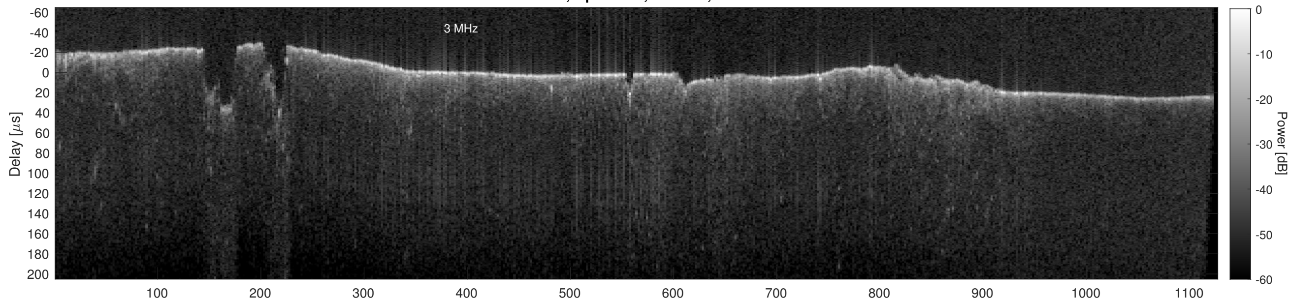
Orbit 16455, Cluttergram
