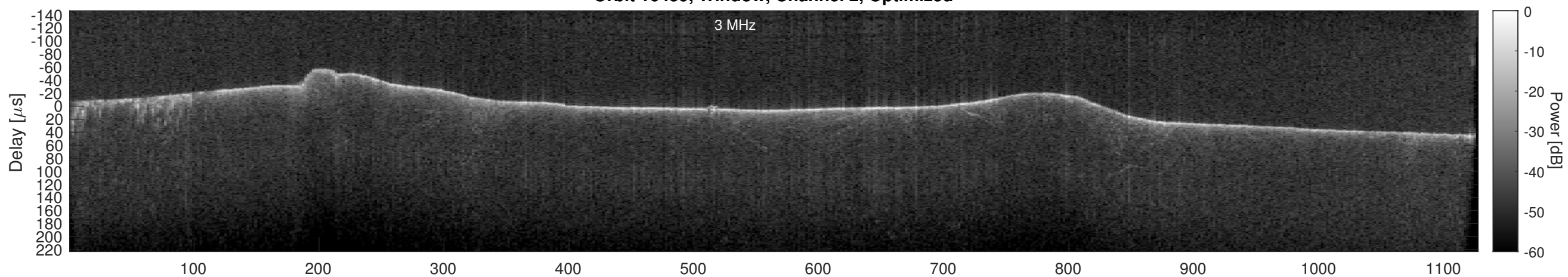
Orbit 16459, Cluttergram
