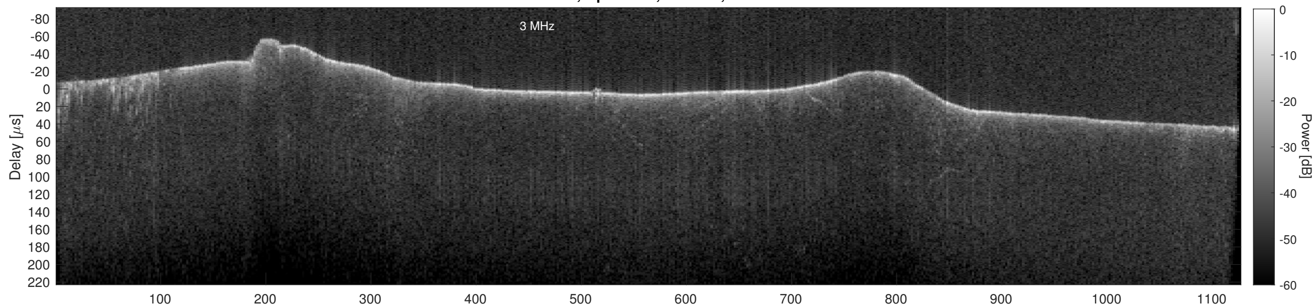
Orbit 16459, Cluttergram
