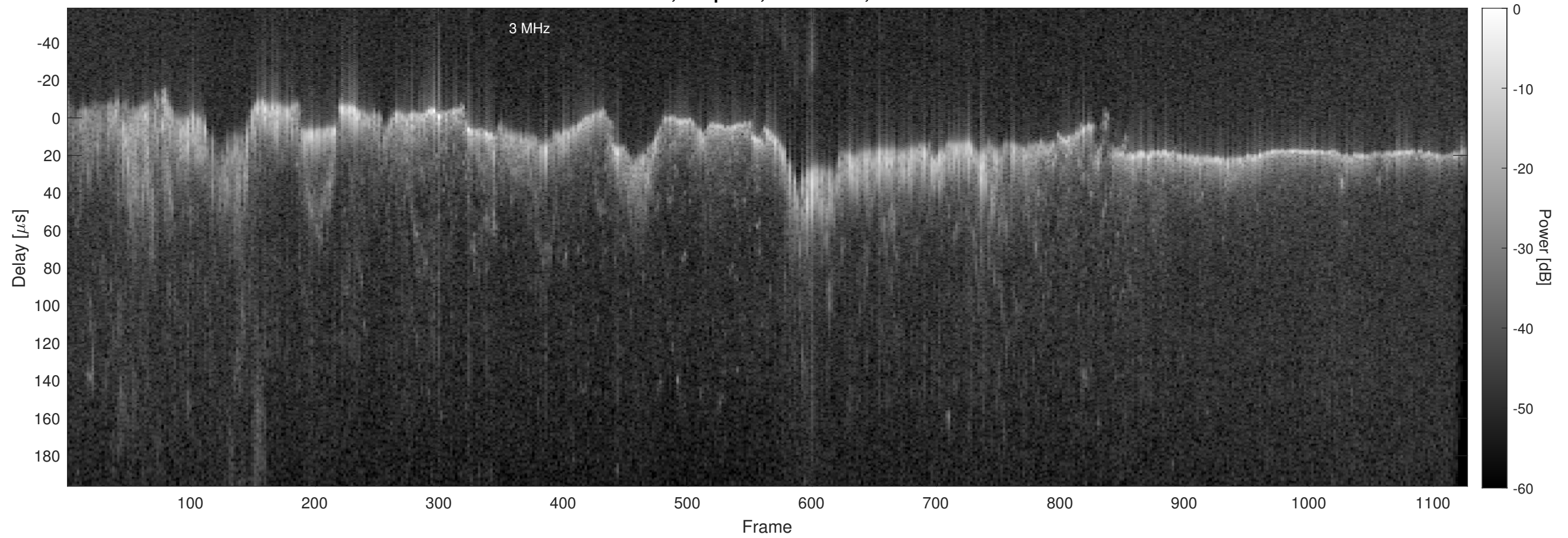
Orbit 16461, Chapman, No Window, Channel 2
