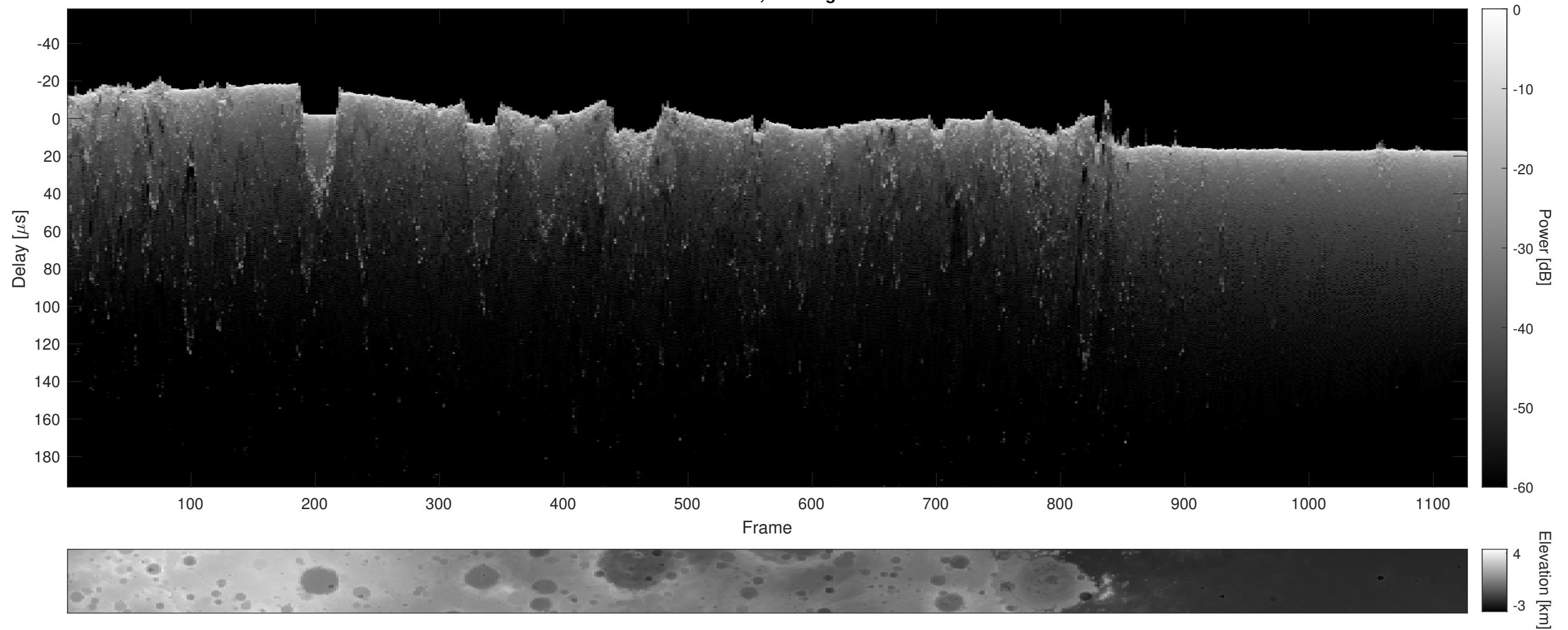
Orbit 16461, Cluttergram
