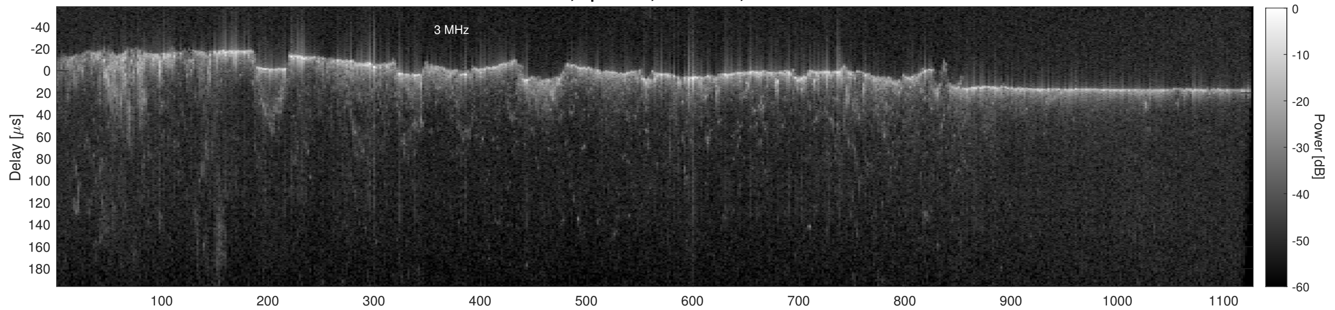
Orbit 16461, Cluttergram
