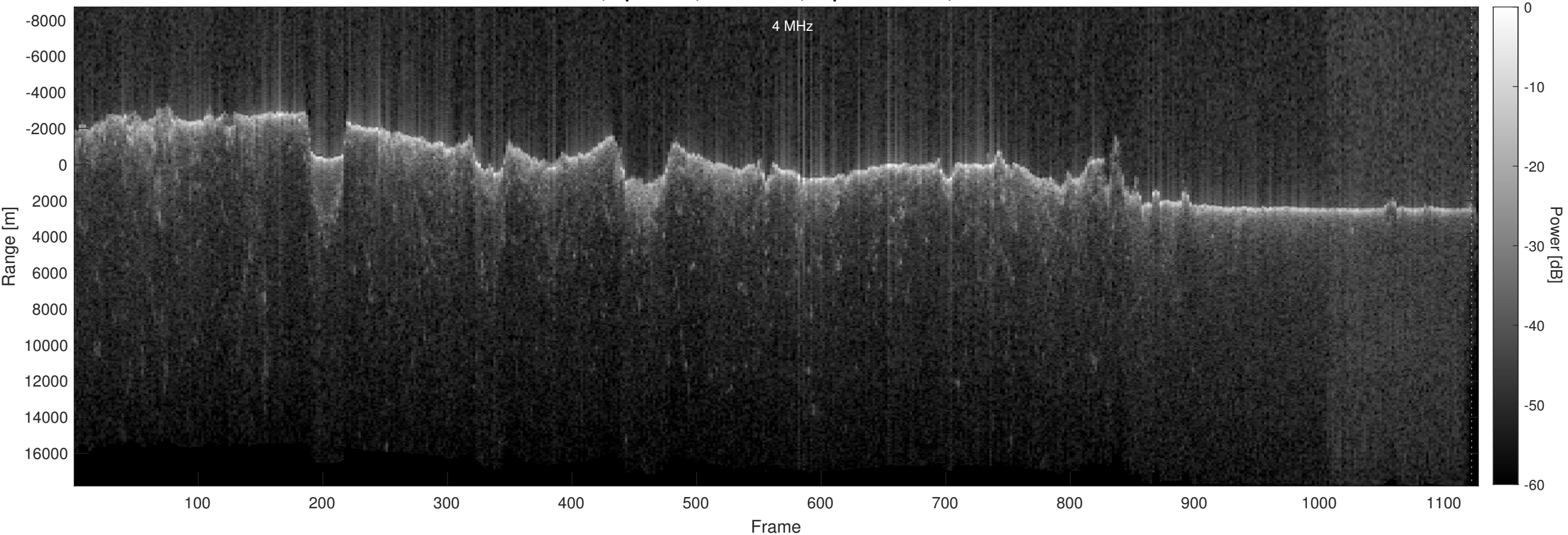
Orbit 16461, Optimized, No Window, Depth-Corrected, Channel 2
