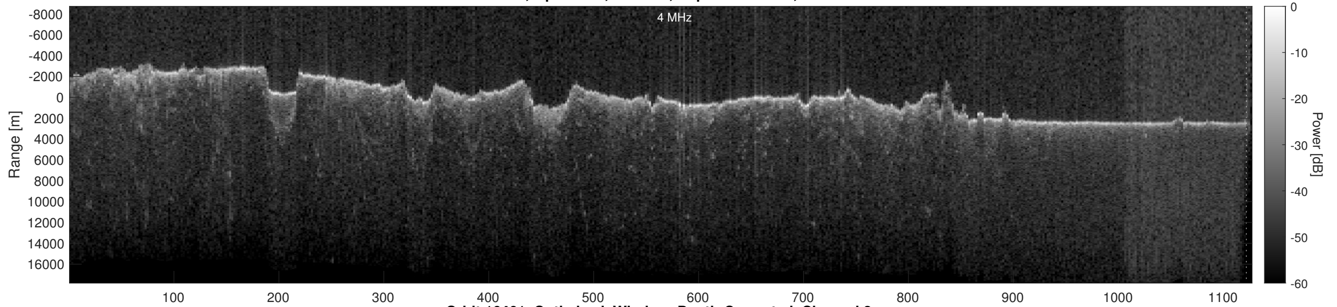
Orbit 16461, Optimized, Window, Depth-Corrected, Channel 2
