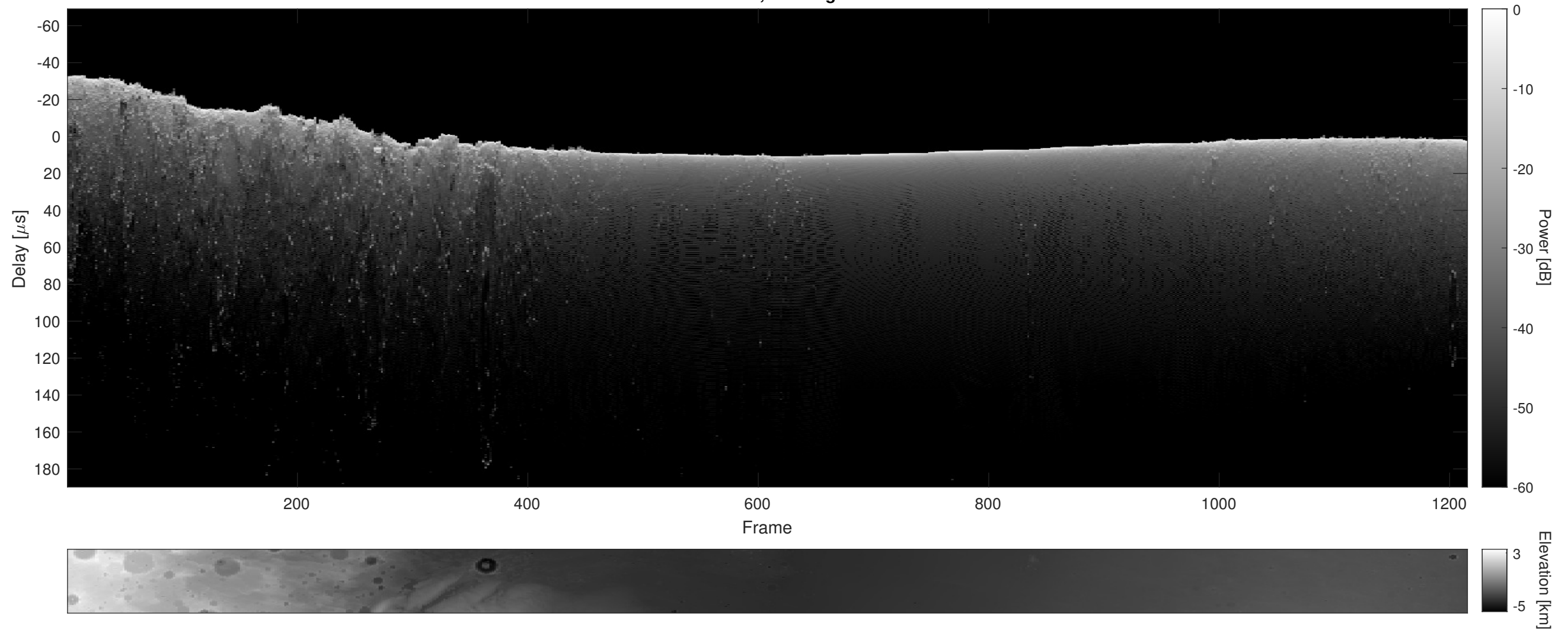
Orbit 16470, Cluttergram
