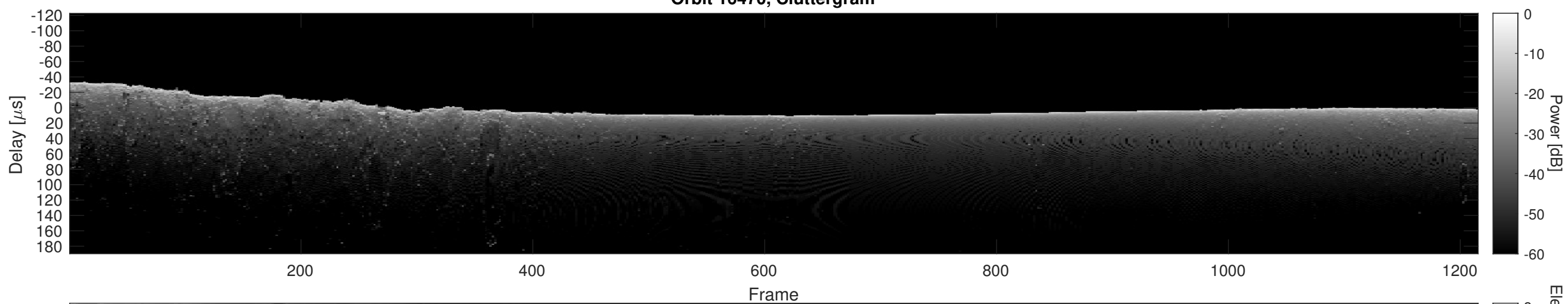
Orbit 16470, Cluttergram
