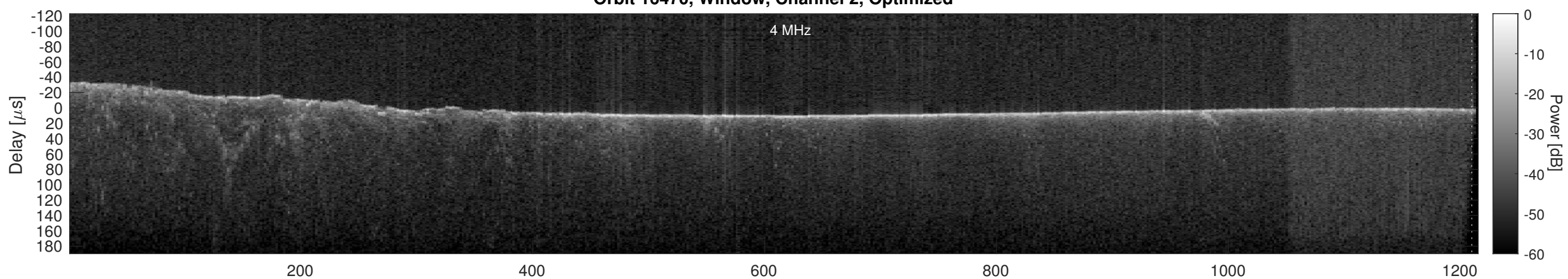
Orbit 16470, Cluttergram
