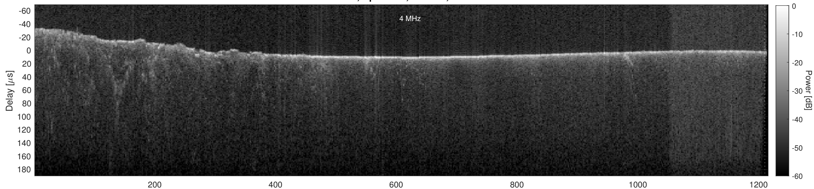
Orbit 16470, Cluttergram
