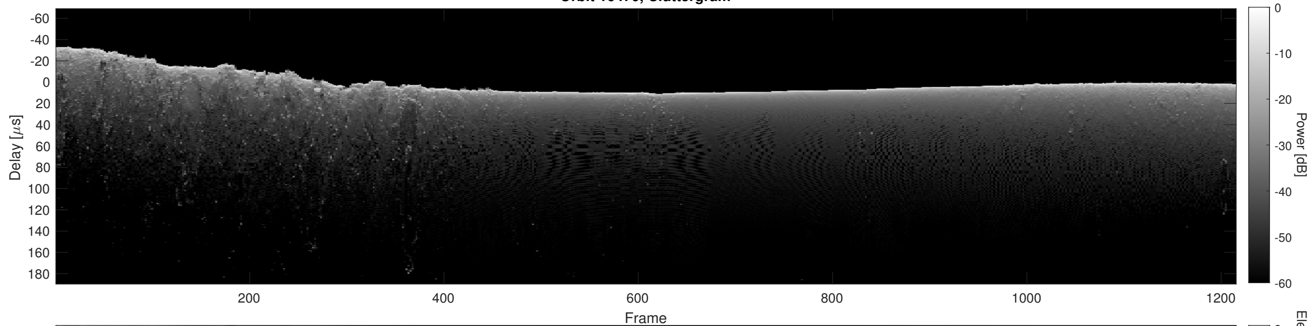
Orbit 16470, Cluttergram
