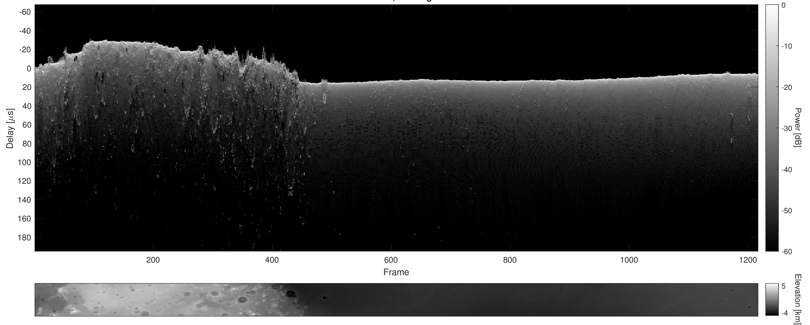
Orbit 16471, Cluttergram
