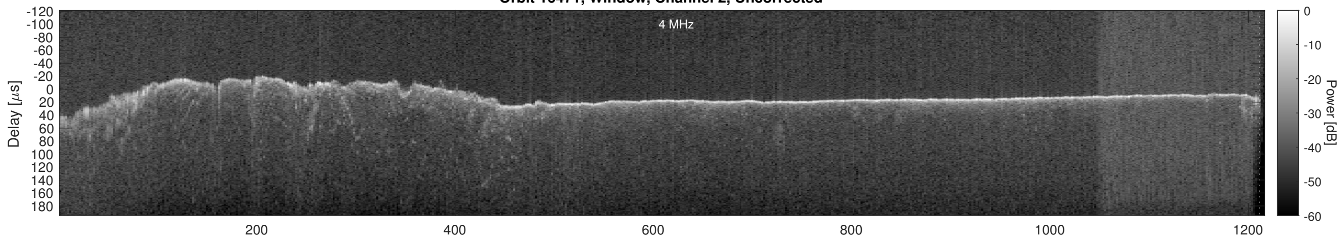
Orbit 16471, Window, Channel 2, Chapman
