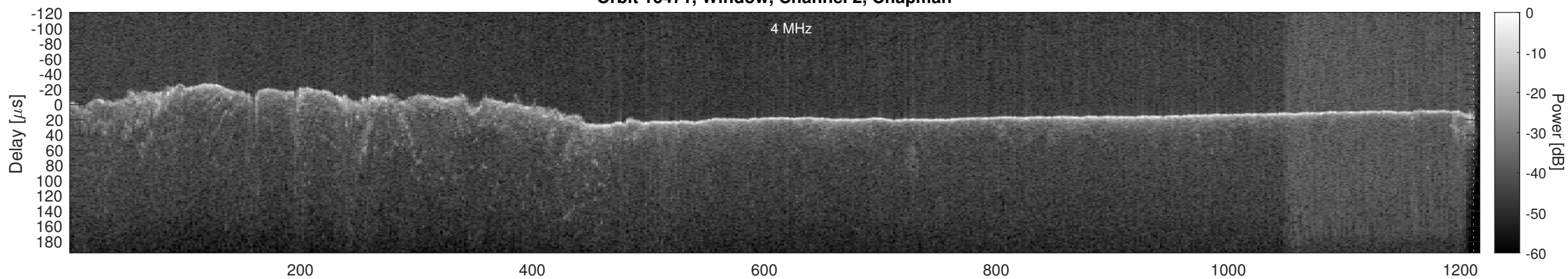
Orbit 16471, Window, Channel 2, Optimized
