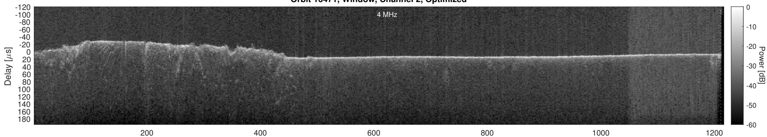
Orbit 16471, Cluttergram
