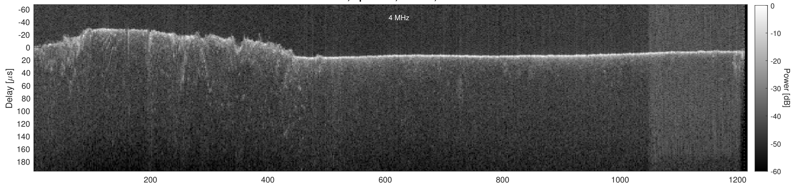
Orbit 16471, Cluttergram
