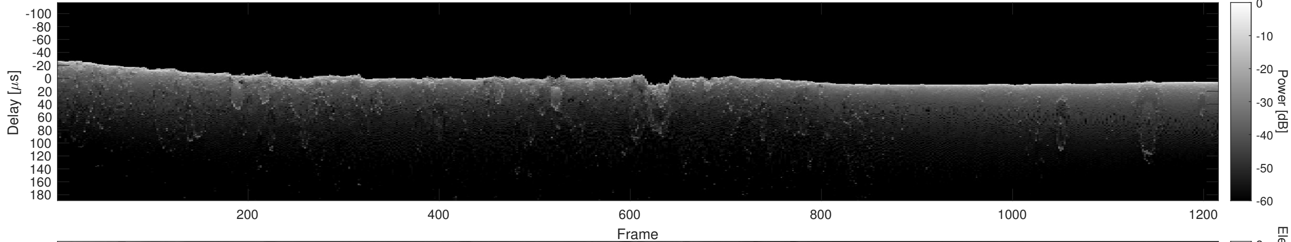
Orbit 16472, Cluttergram
