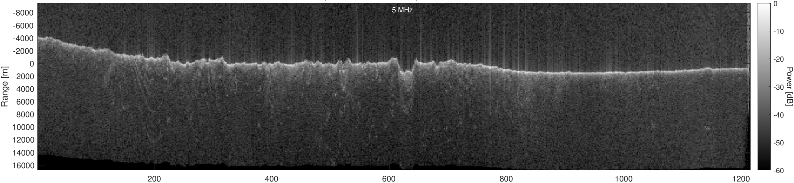
Orbit 16472, Optimized, Window, Depth-Corrected, Channel 2
