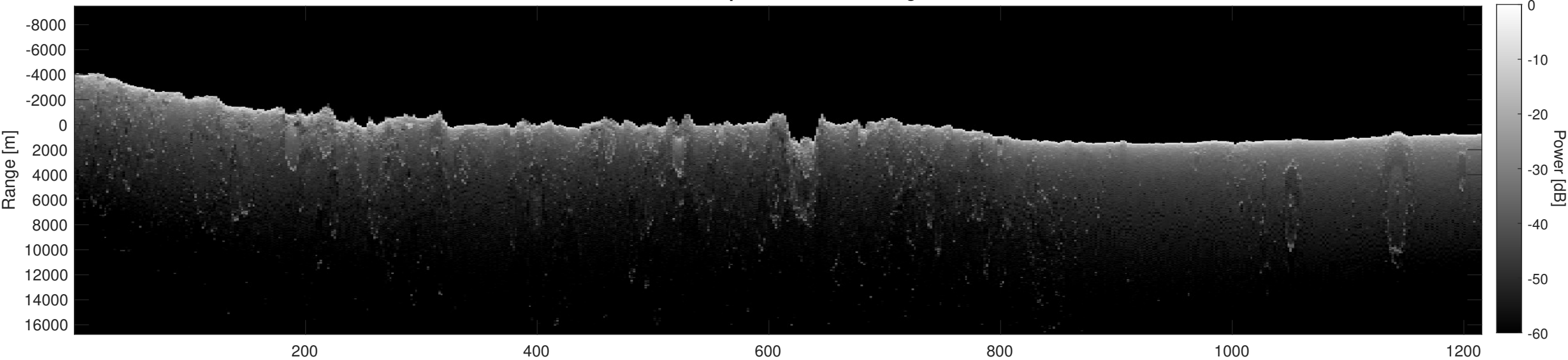
Orbit 16472, Depth-Corrected Cluttergram
