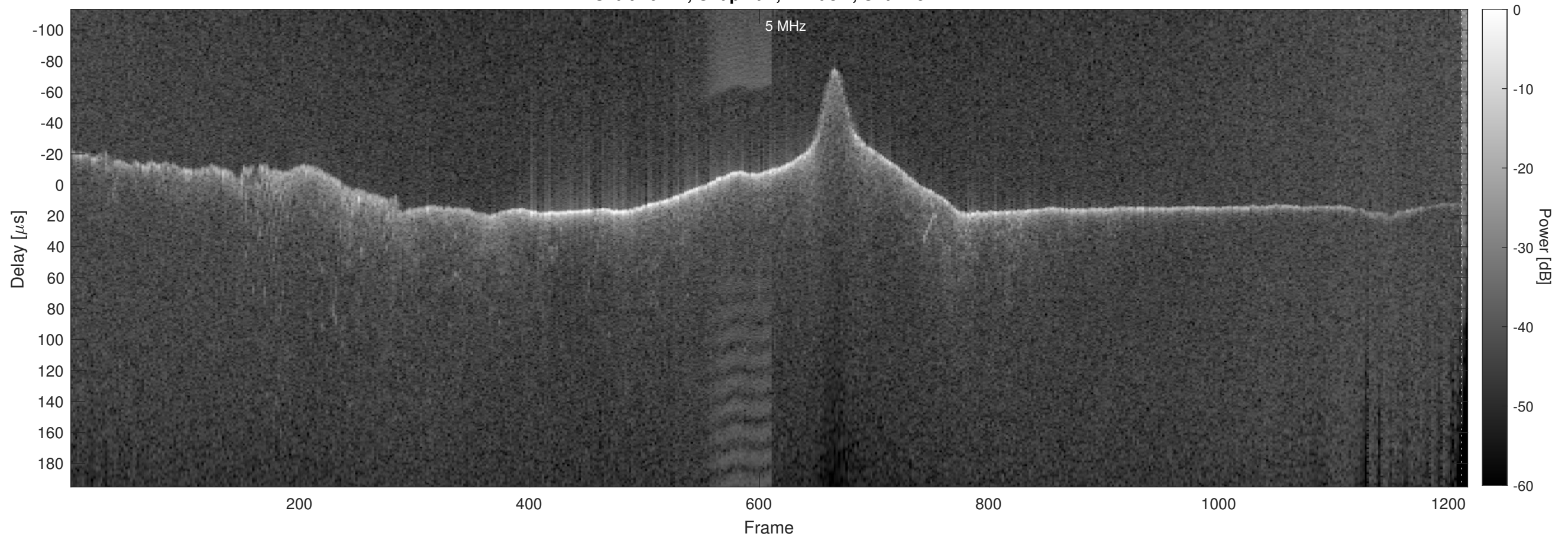
Orbit 16474, Chapman, Window, Channel 2
