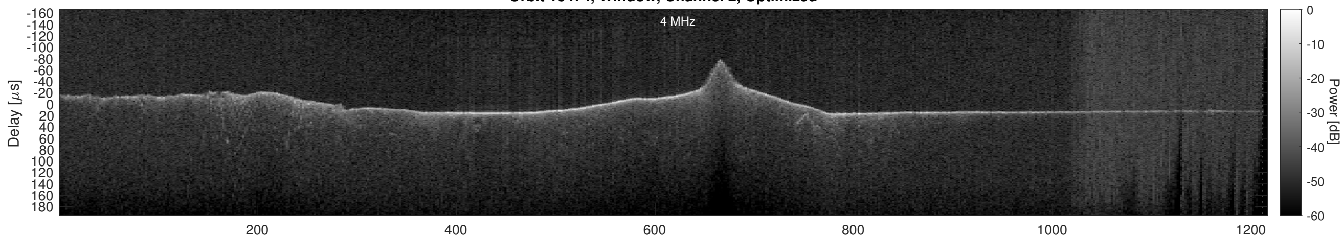
Orbit 16474, Cluttergram
