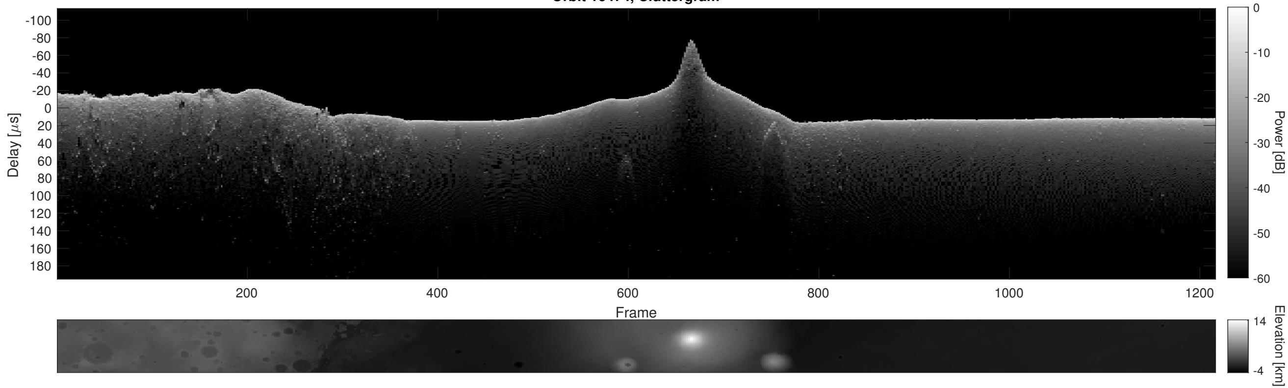
Orbit 16474, Cluttergram
