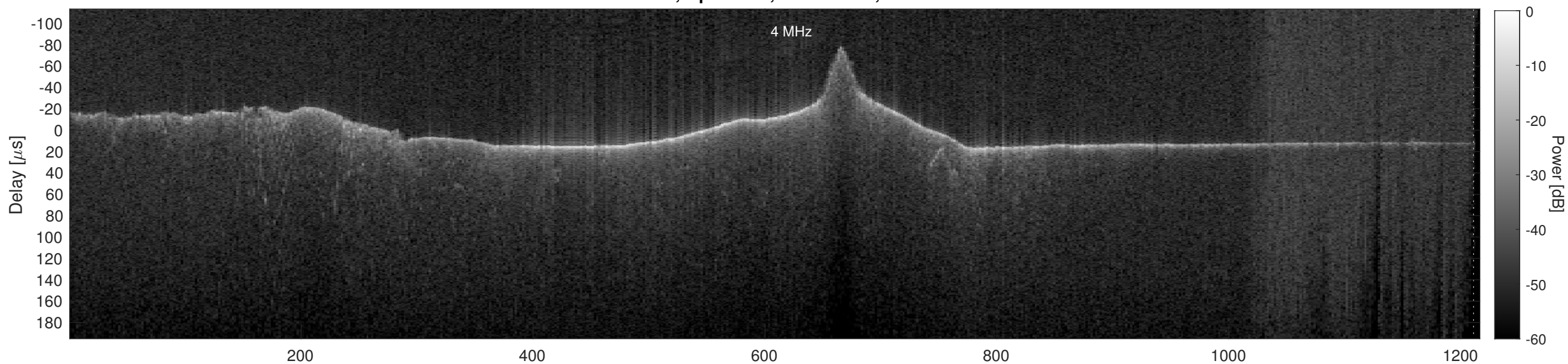
Orbit 16474, Cluttergram
