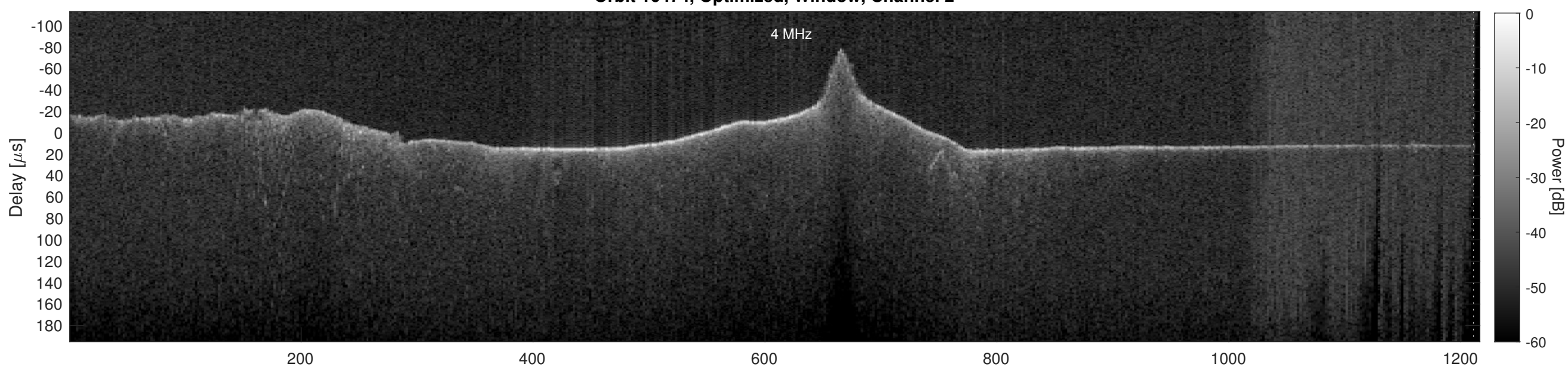
Orbit 16474, Cluttergram
