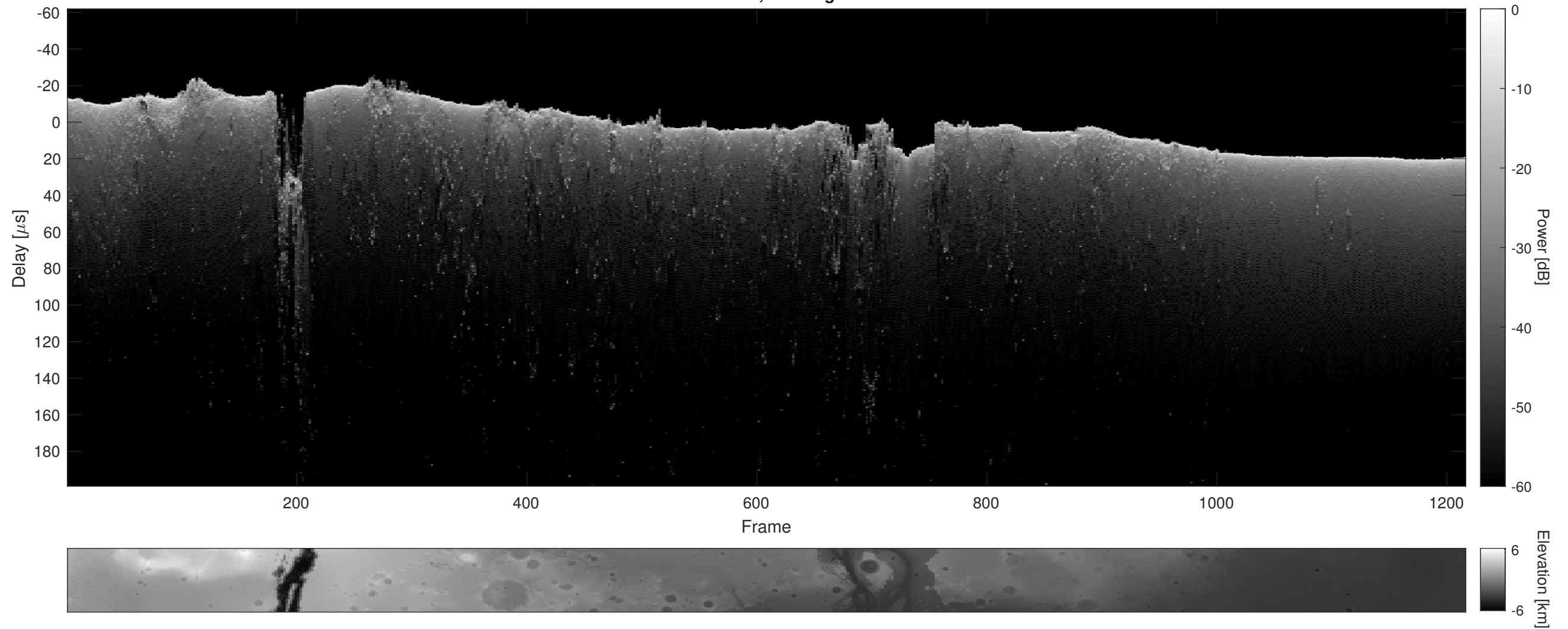
Orbit 16476, Cluttergram
