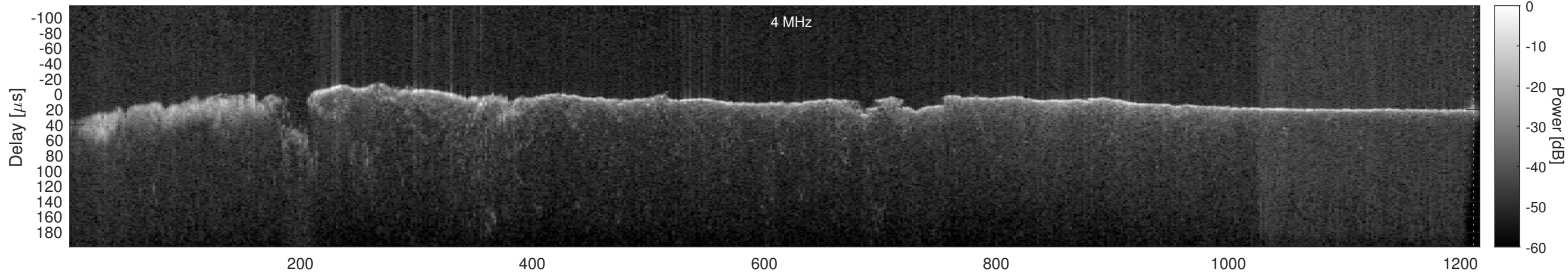
Orbit 16476, Window, Channel 2, Chapman
