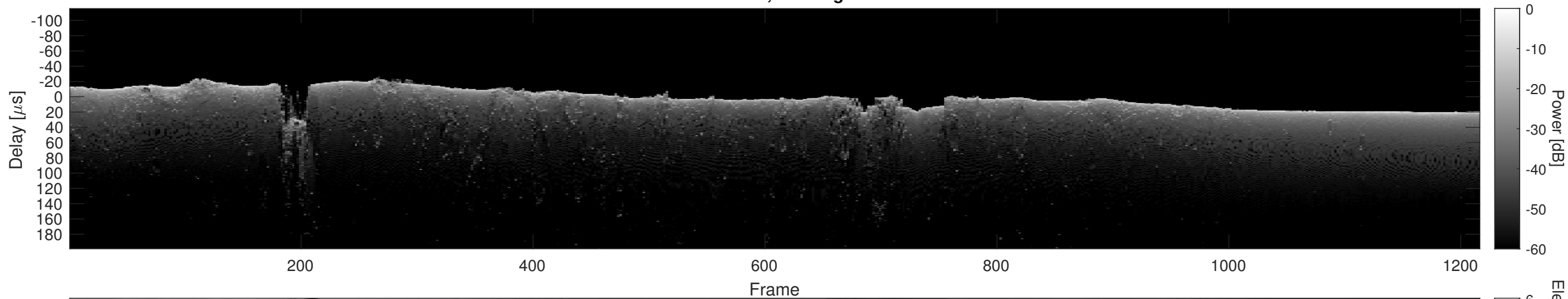
Orbit 16476, Cluttergram
