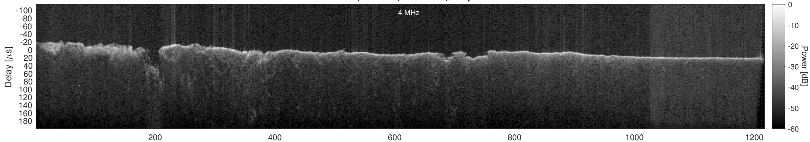
Orbit 16476, Window, Channel 2, Optimized
