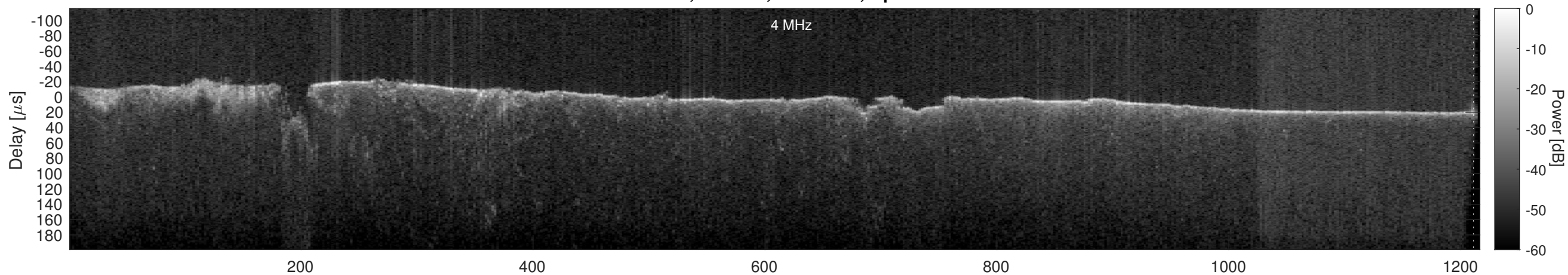
Orbit 16476, Cluttergram
