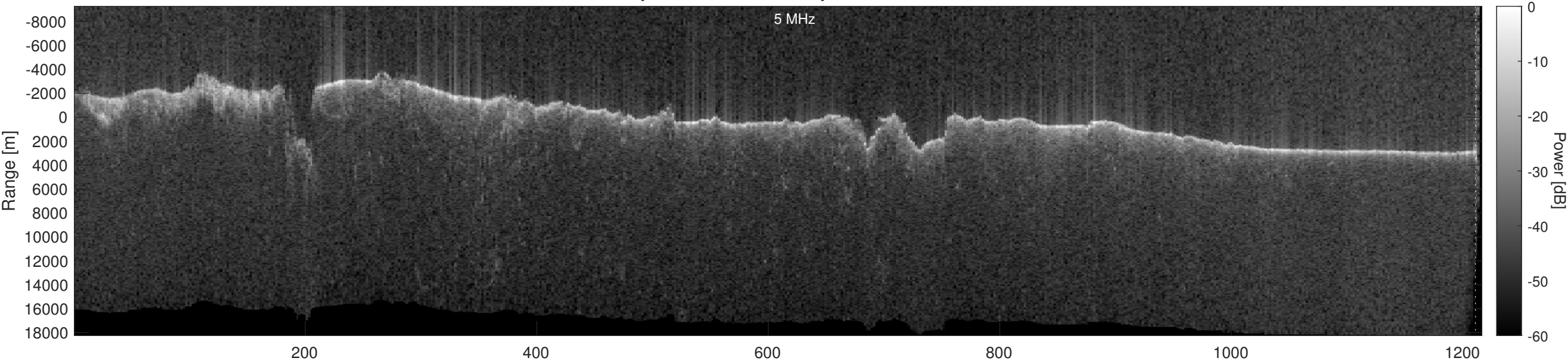
Orbit 16476, Optimized, Window, Depth-Corrected, Channel 2
