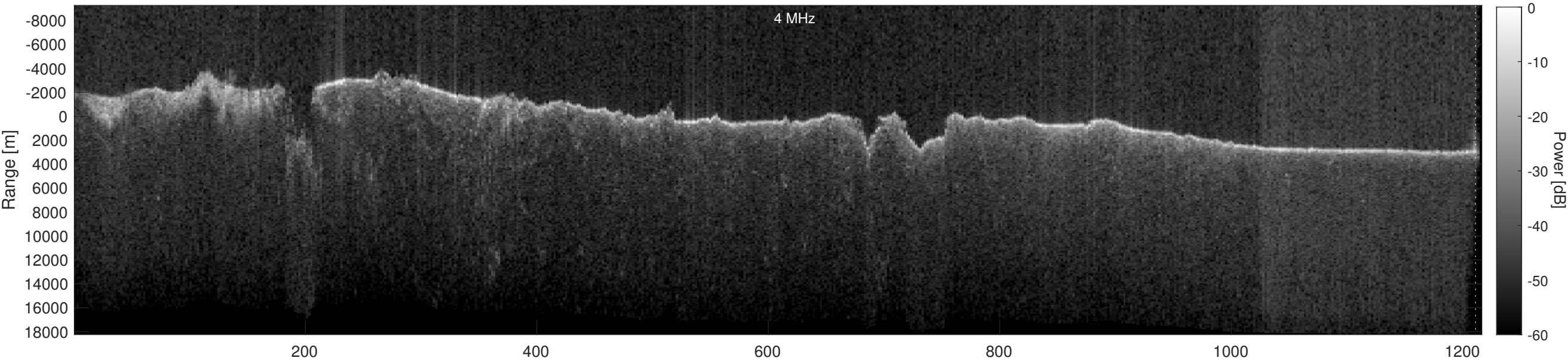
Orbit 16476, Depth-Corrected Cluttergram
