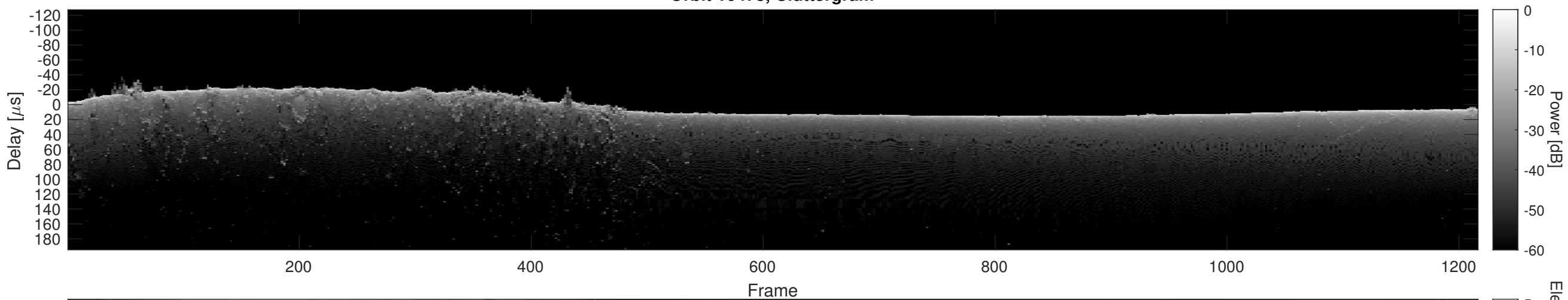
Orbit 16478, Cluttergram
