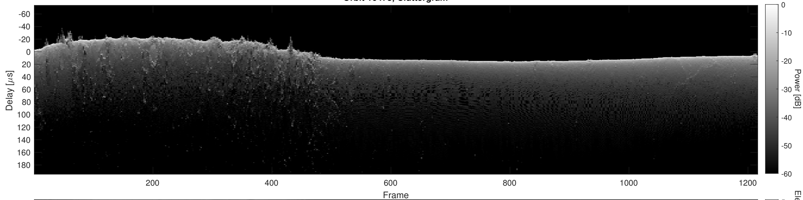
Orbit 16478, Cluttergram
