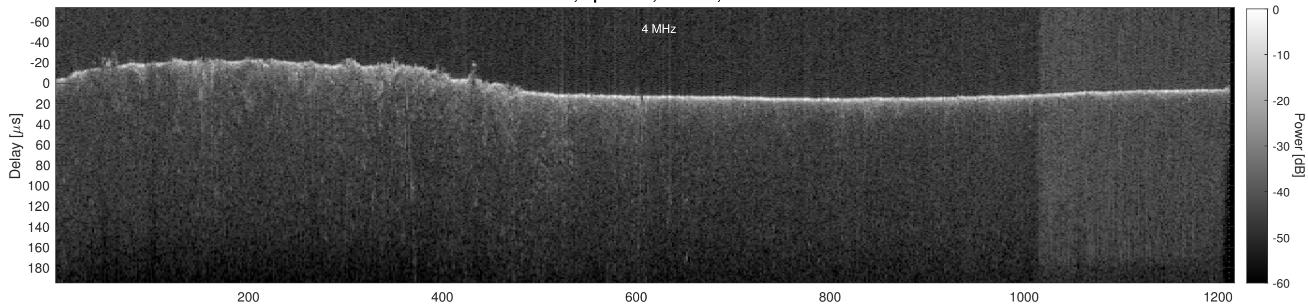
Orbit 16478, Cluttergram
