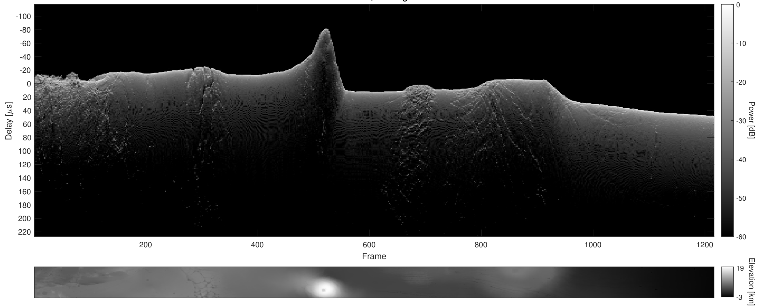
Orbit 16480, Cluttergram
