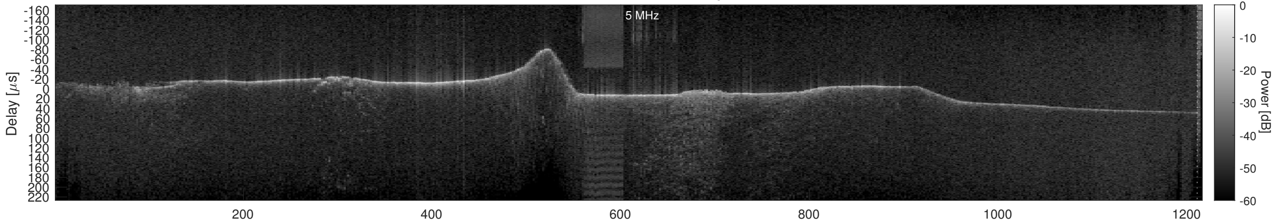
Orbit 16480, Cluttergram
