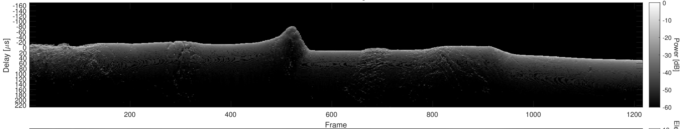
Orbit 16480, Cluttergram
