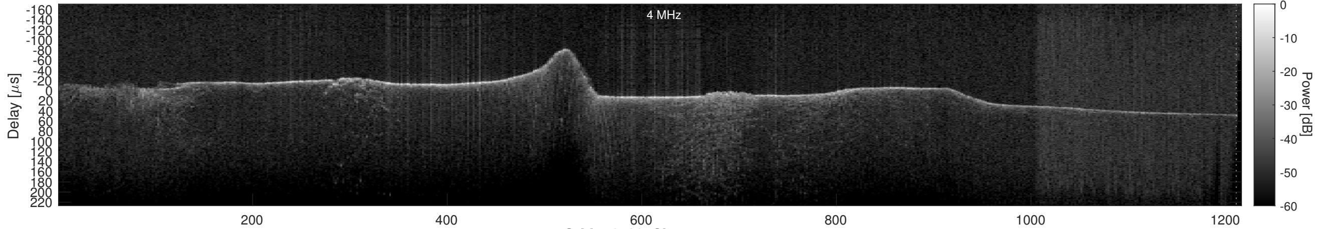
Orbit 16480, Cluttergram
