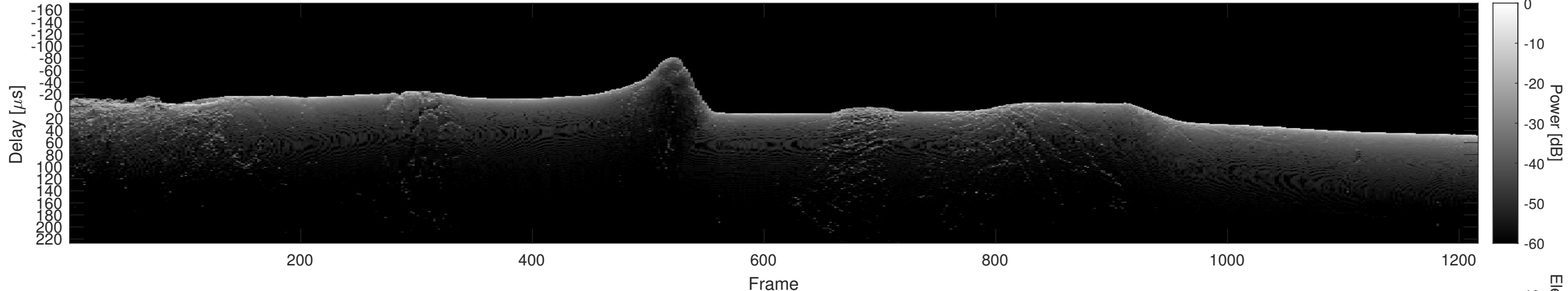
Orbit 16480, Cluttergram
