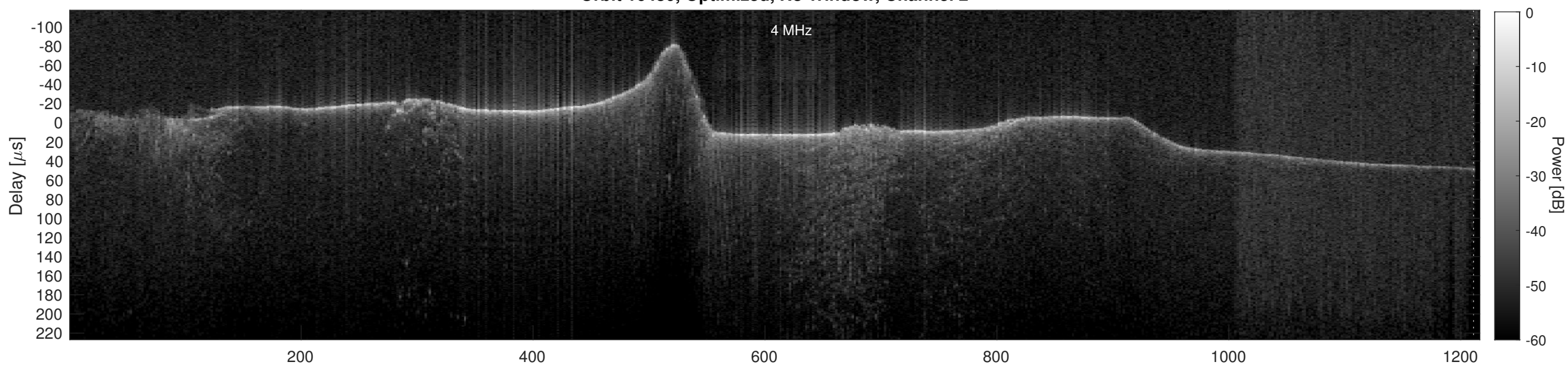
Orbit 16480, Cluttergram
