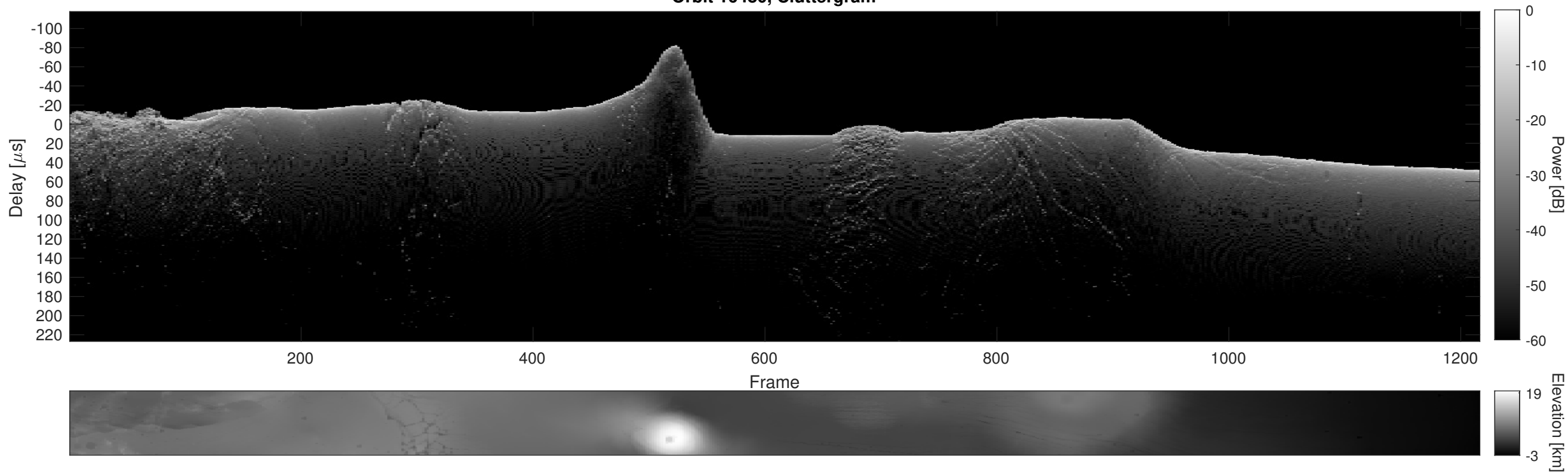
Orbit 16480, Cluttergram
