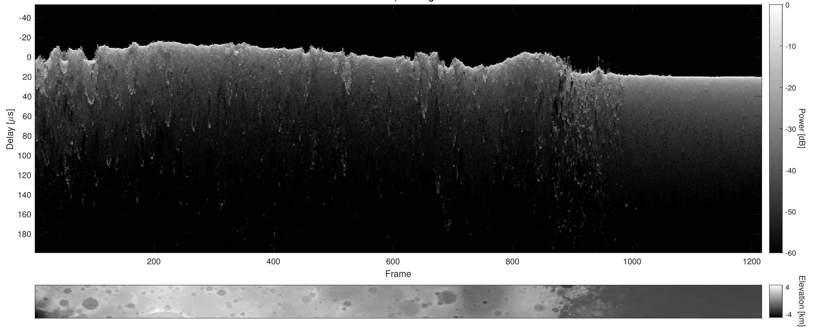
Orbit 16482, Cluttergram
