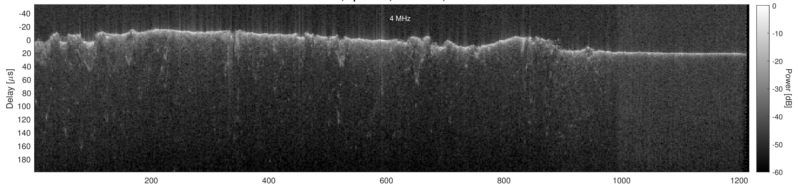
Orbit 16482, Cluttergram
