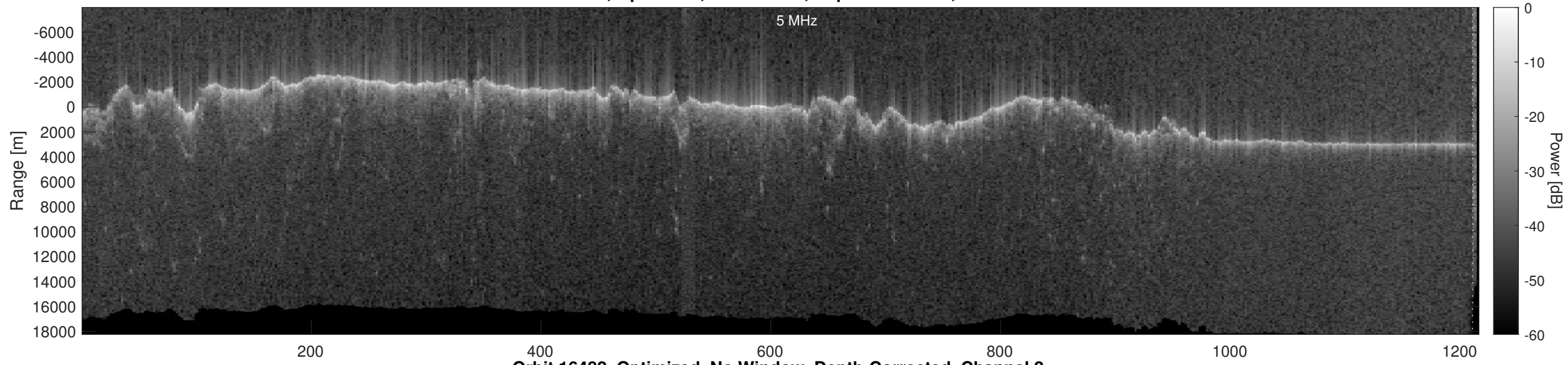
Orbit 16482, Optimized, No Window, Depth-Corrected, Channel 2
