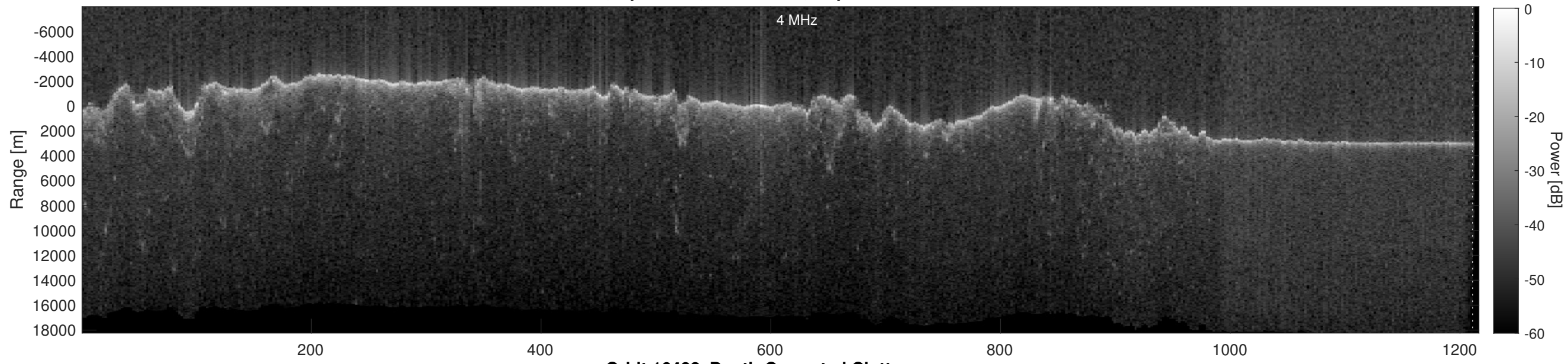
Orbit 16482, Depth-Corrected Cluttergram
