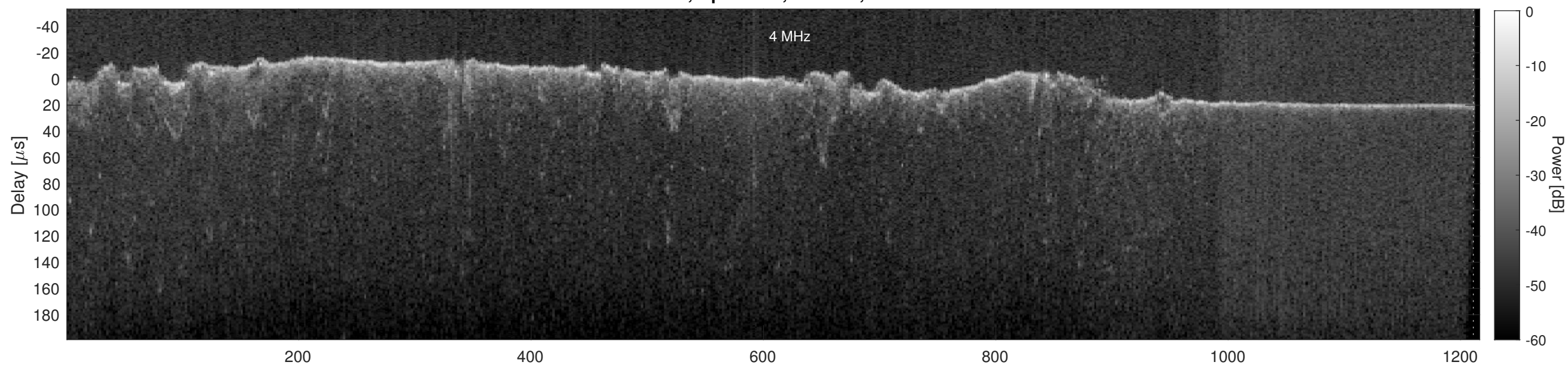
Orbit 16482, Cluttergram
