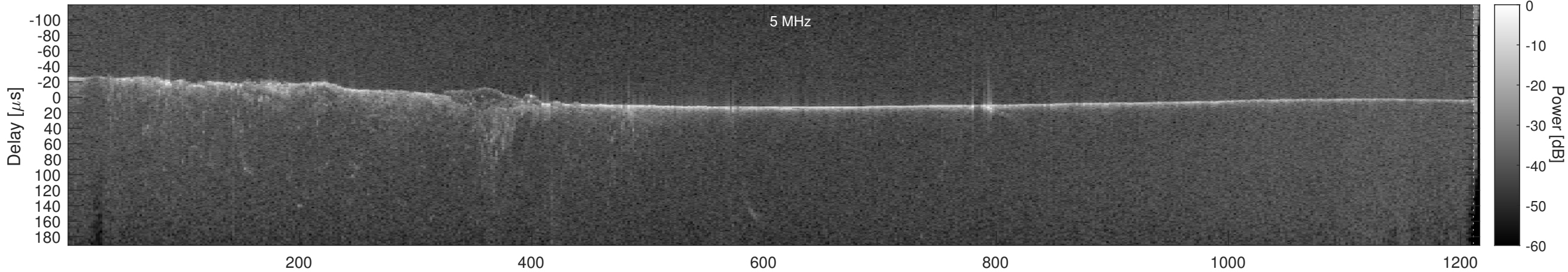
Orbit 16484, Cluttergram
