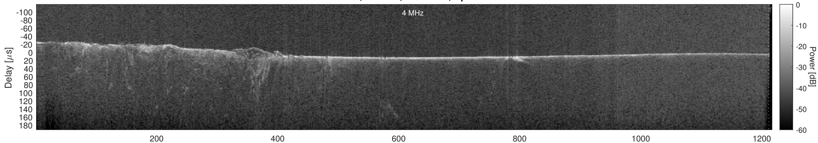
Orbit 16484, Cluttergram
