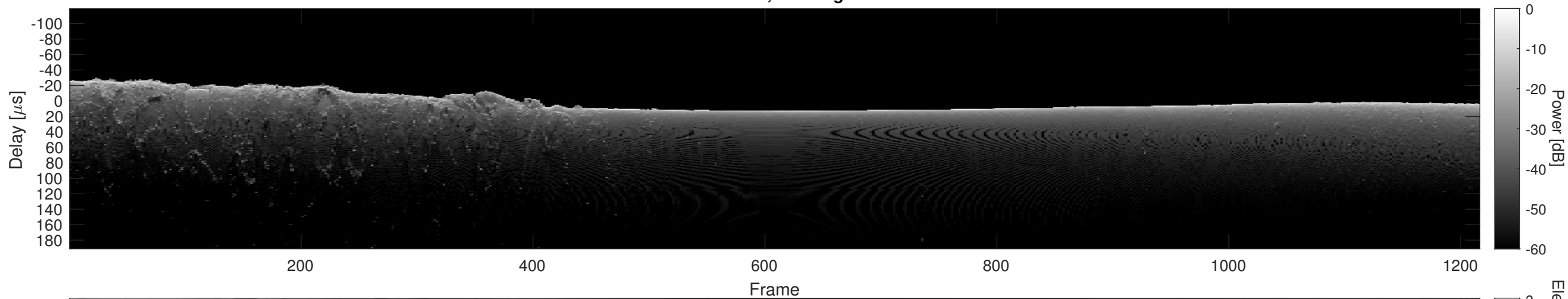
Orbit 16484, Cluttergram
