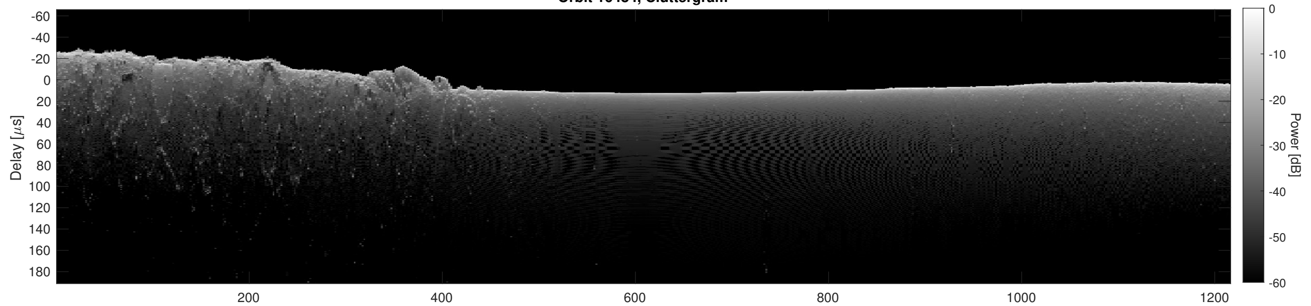
Orbit 16484, Cluttergram
