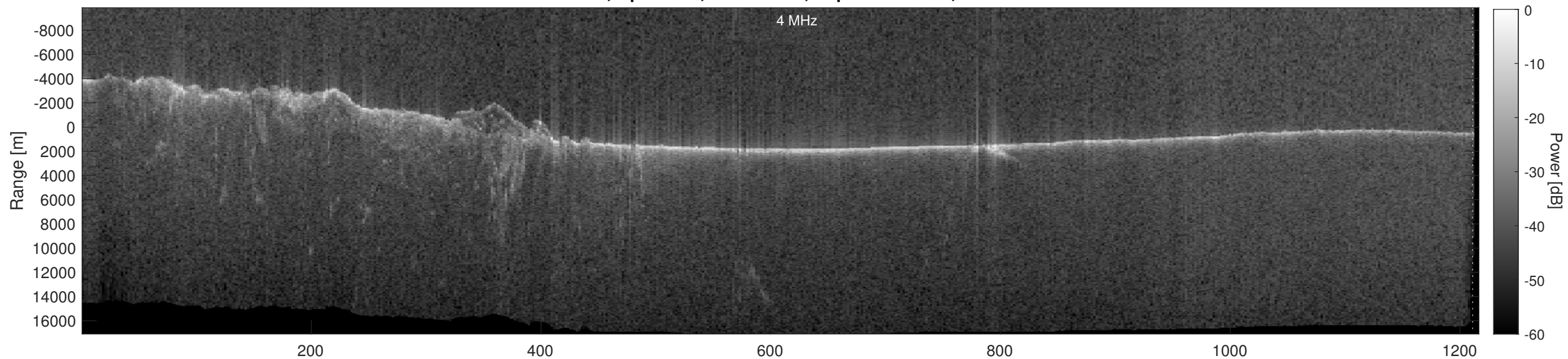
Orbit 16484, Depth-Corrected Cluttergram
