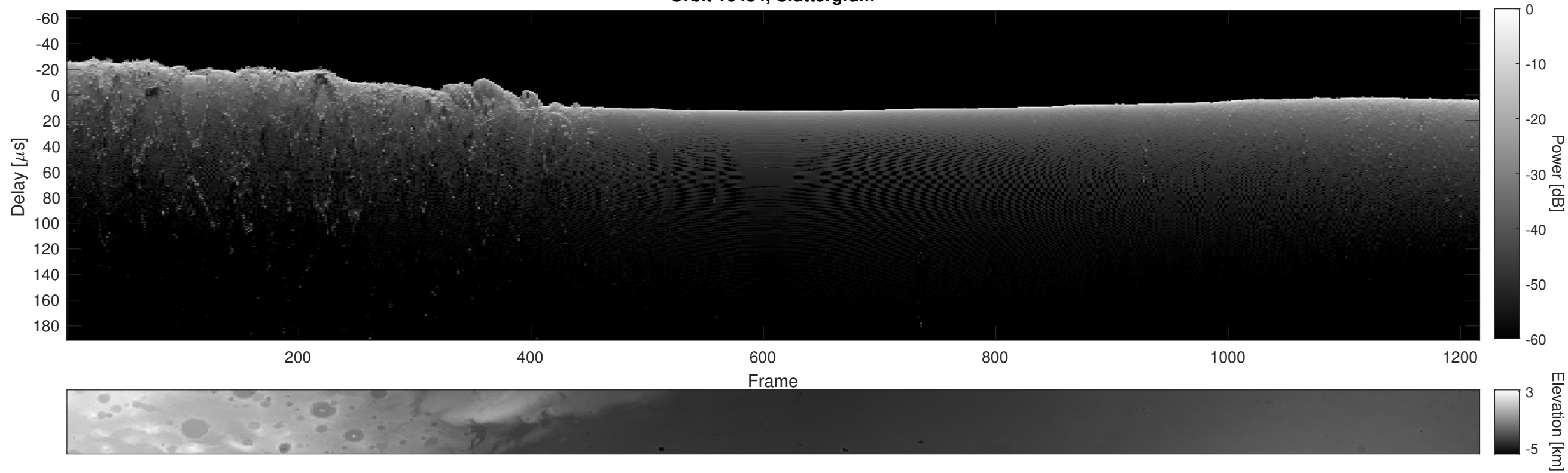
Orbit 16484, Cluttergram
