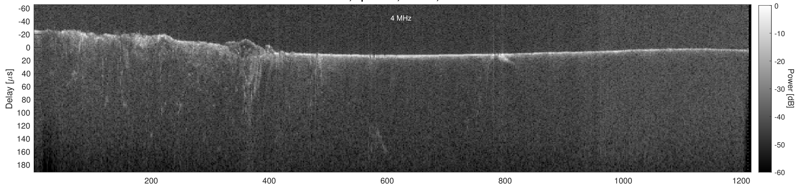
Orbit 16484, Cluttergram
