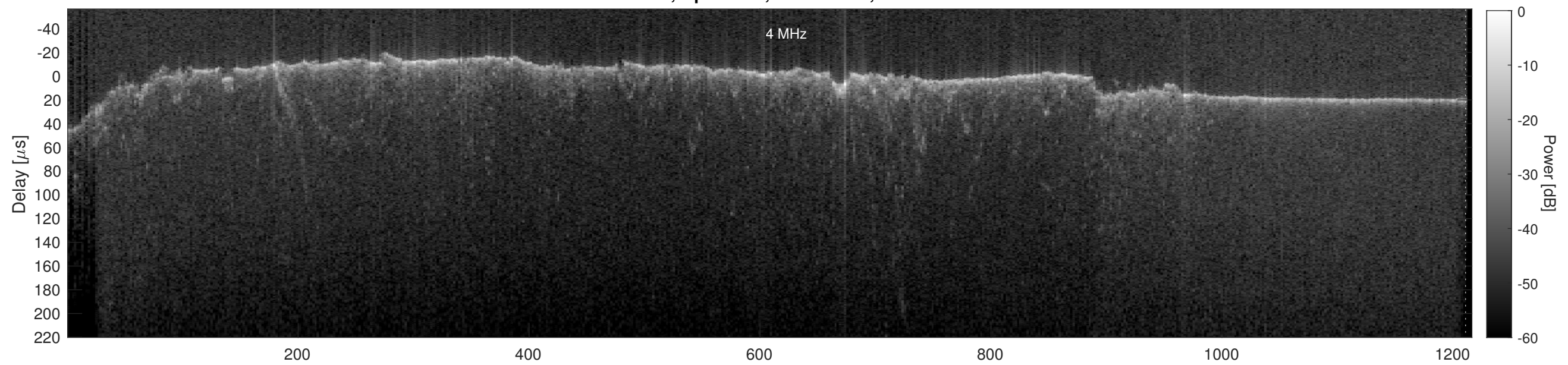
Orbit 16489, Cluttergram
