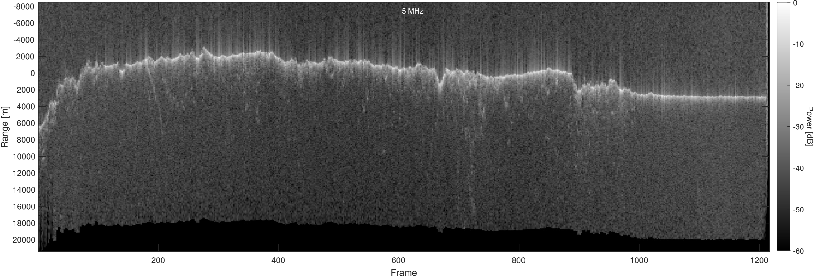
Orbit 16489, Optimized, No Window, Depth-Corrected, Channel 2
