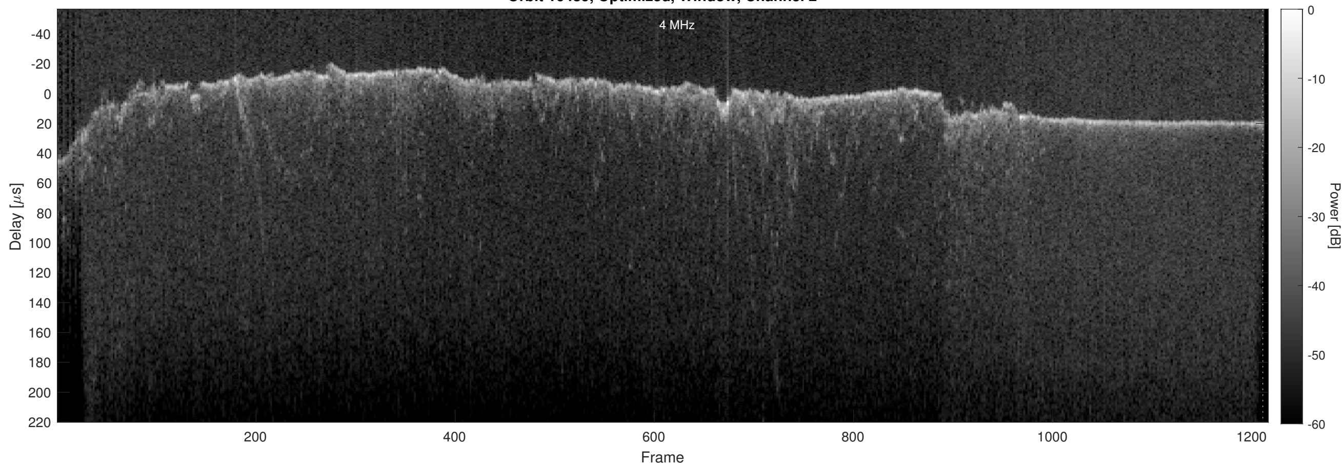
Orbit 16489, Optimized, Window, Channel 2
