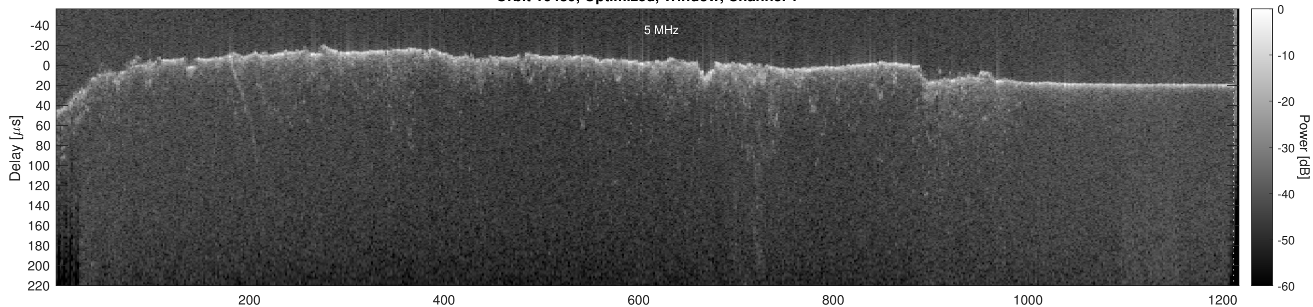
Orbit 16489, Optimized, Window, Channel 2
