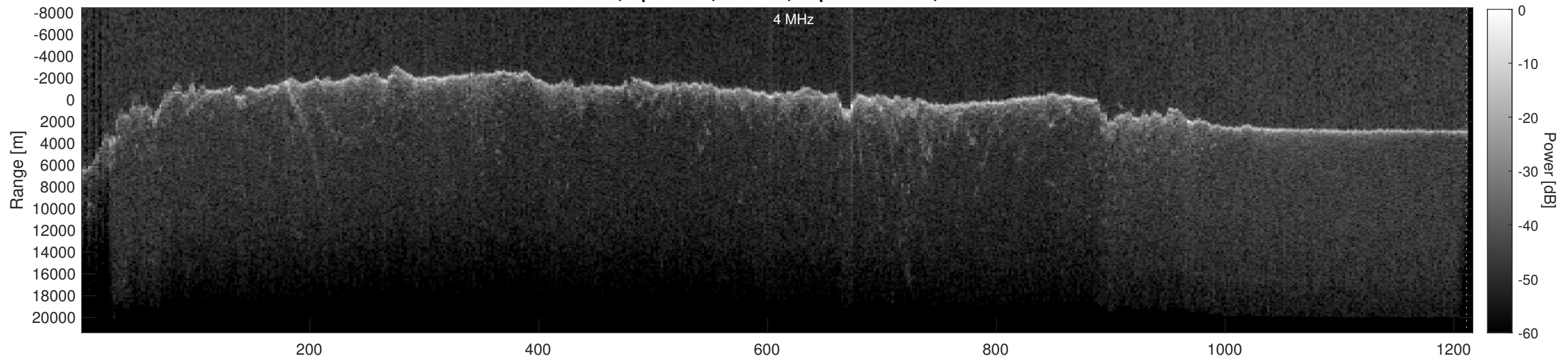
Orbit 16489, Depth-Corrected Cluttergram
