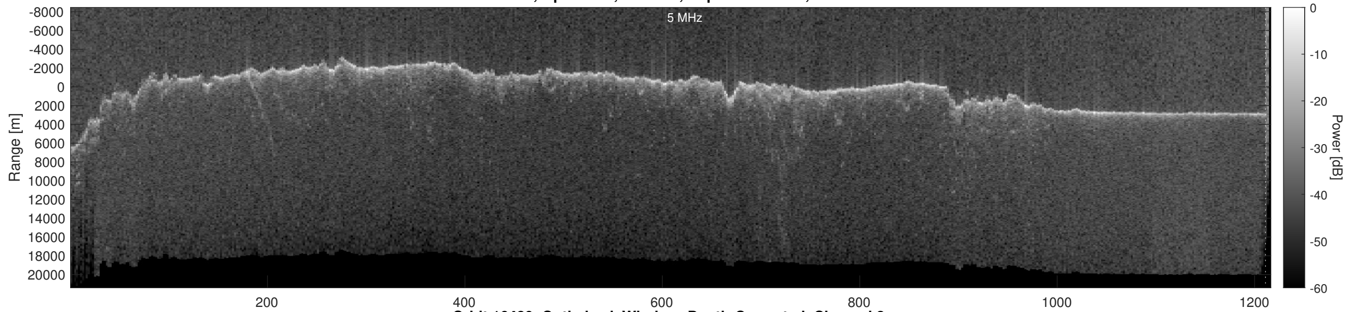
Orbit 16489, Optimized, Window, Depth-Corrected, Channel 2
