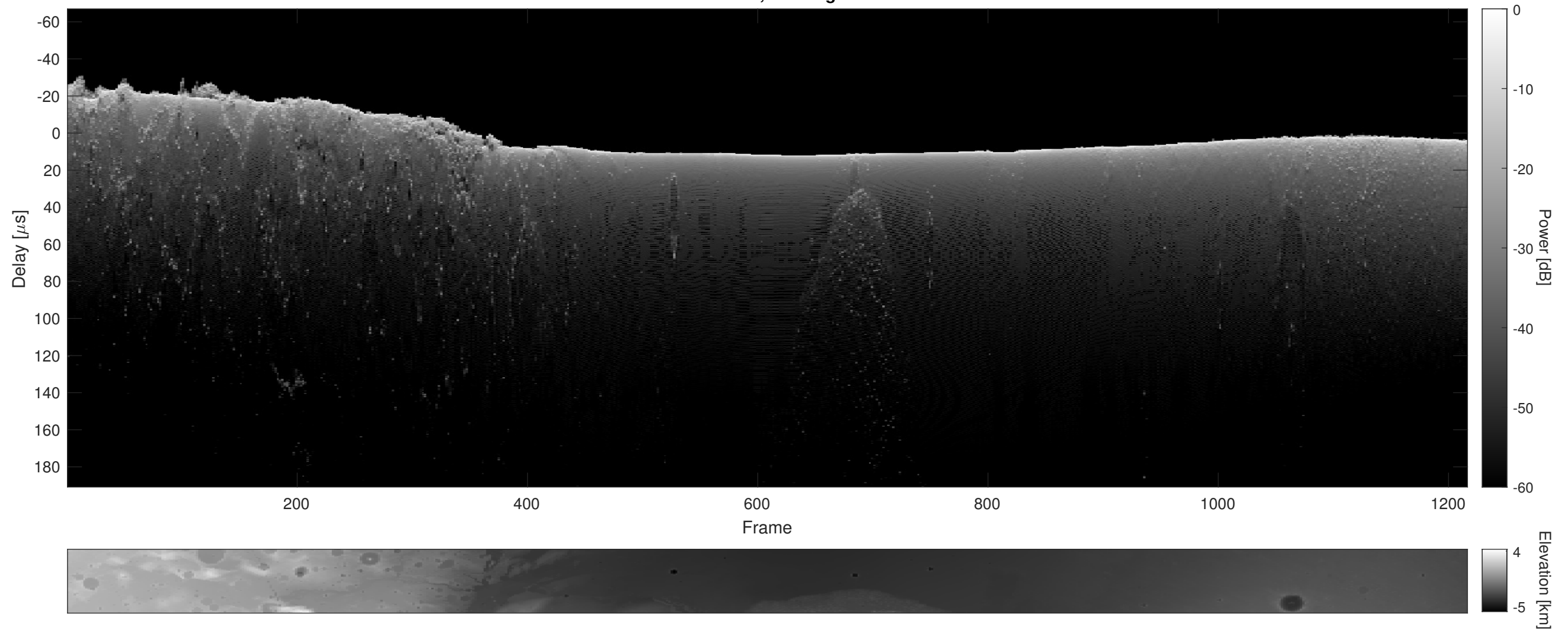
Orbit 16491, Cluttergram
