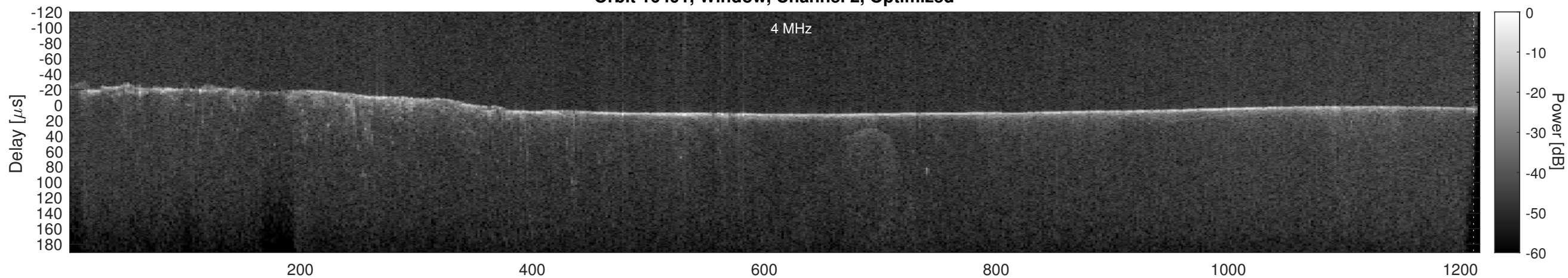
Orbit 16491, Cluttergram
