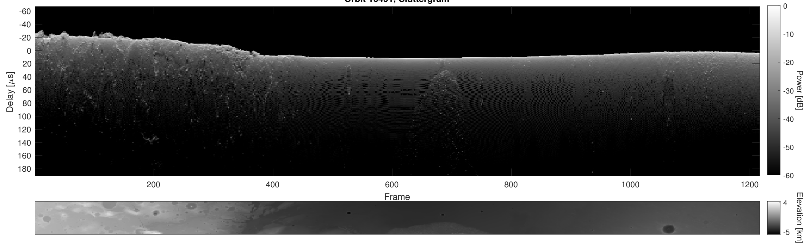
Orbit 16491, Cluttergram
