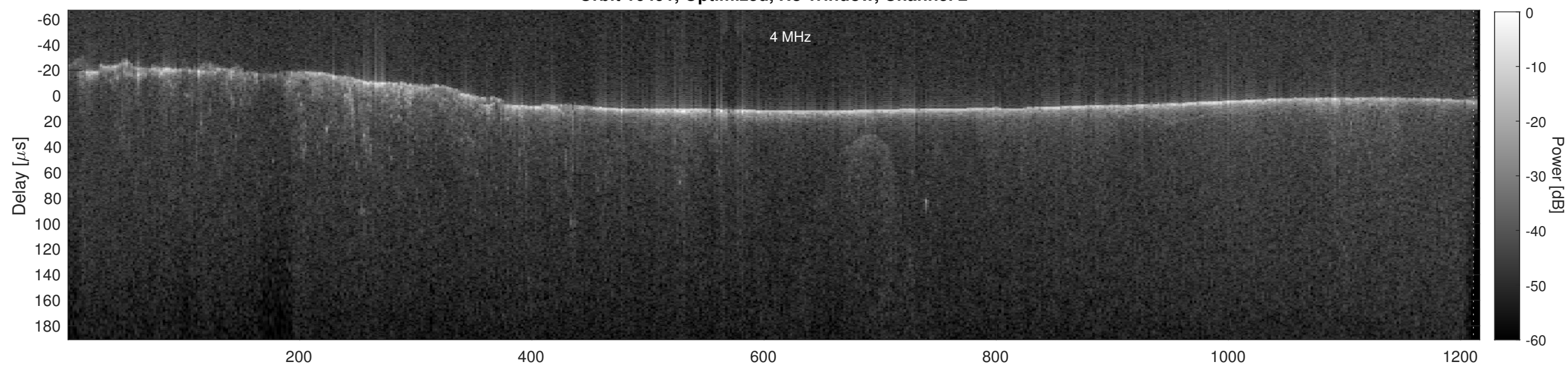
Orbit 16491, Cluttergram
