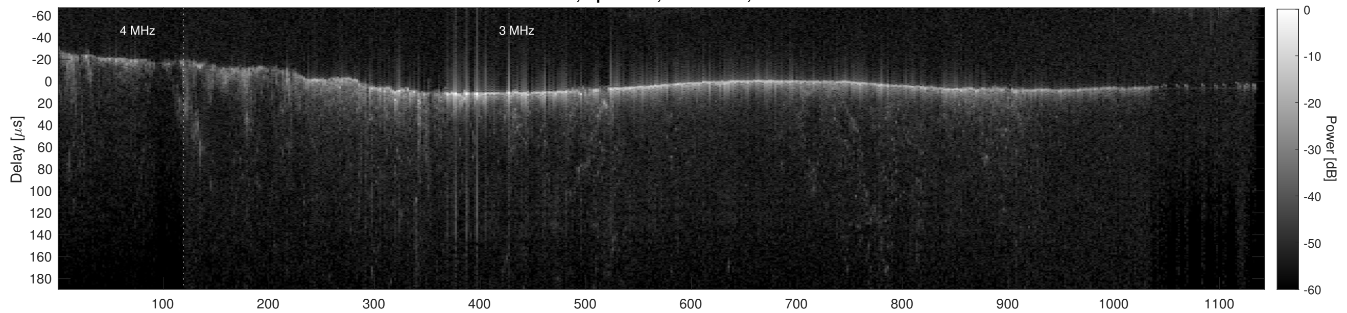
Orbit 16495, Cluttergram
