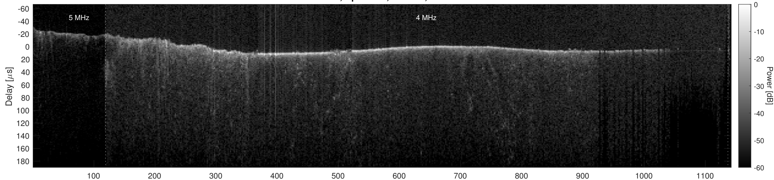
Orbit 16495, Optimized, Window, Channel 2
