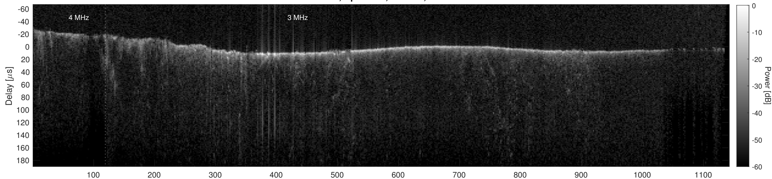
Orbit 16495, Cluttergram
