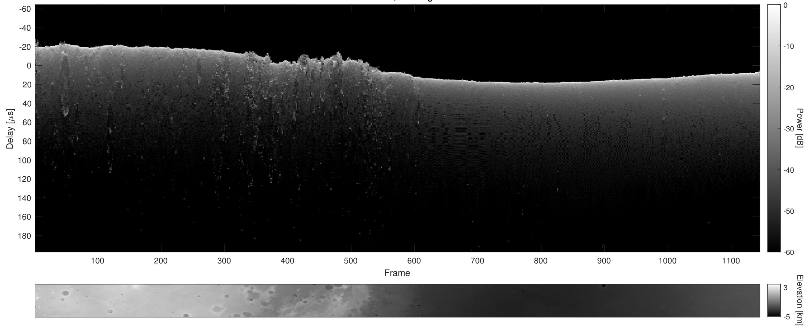
Orbit 16499, Cluttergram
